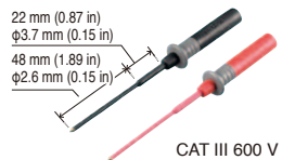
BREAKER PIN SET L4939
