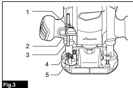
Fig. 3 ► 1. Depth pointer 2. Screw 3. Stopper pole 4. Adjusting hex bolt 5. Stopper block
