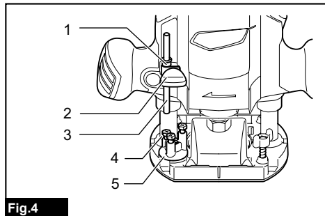
Fig. 4 ► 1. Depth pointer 2. Screw 3. Stopper pole 4. Adjusting hex bolt 5. Stopper block
